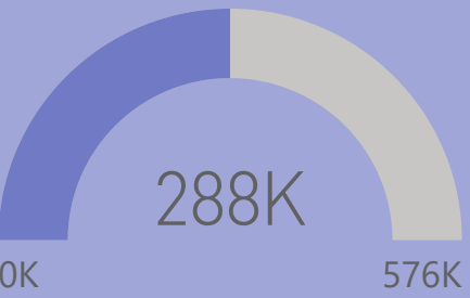
Successful_Transactions
