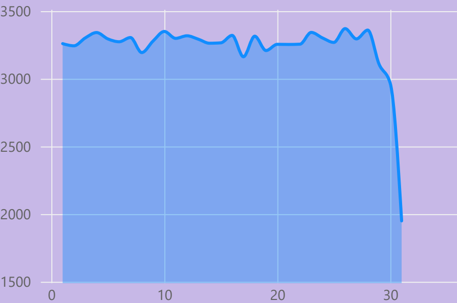
Active_Users
