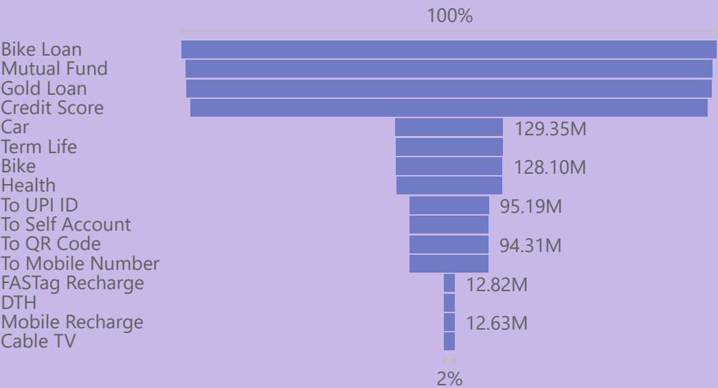
Failed_Transactions
