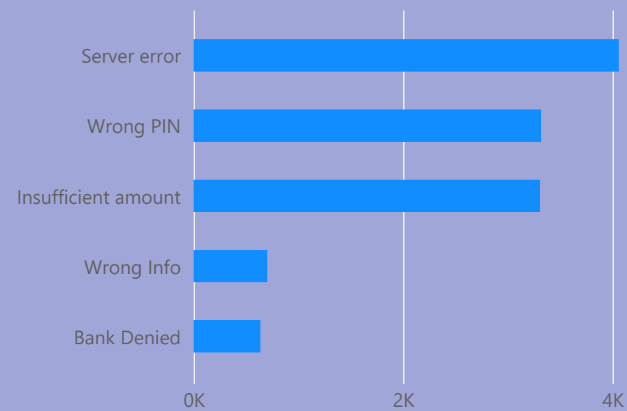
Failed_Transactions
