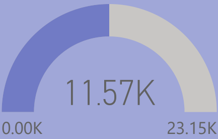
Avg_Transaction_Value
