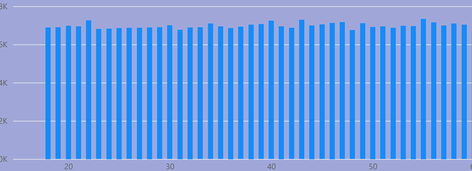
Total_Transactions
