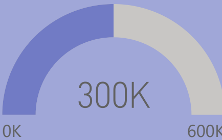
Total_Transactions
