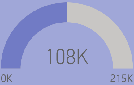
Total_Users
