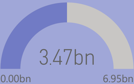
Total_Amount
